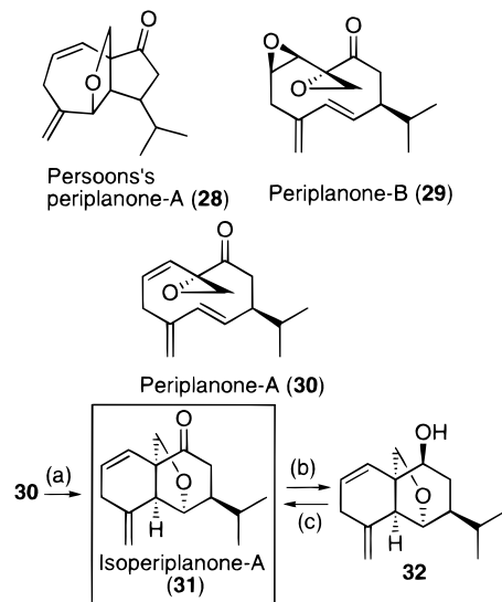
Scheme 6. Synthesis of Persoons's Periplanone-A (= Isoperiplanone-A) a
